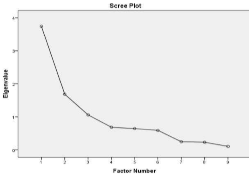
Figure 1. Eigenvalue Graph
